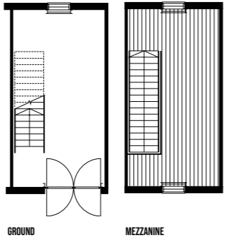
Type 2b - 688 sq.ft.
